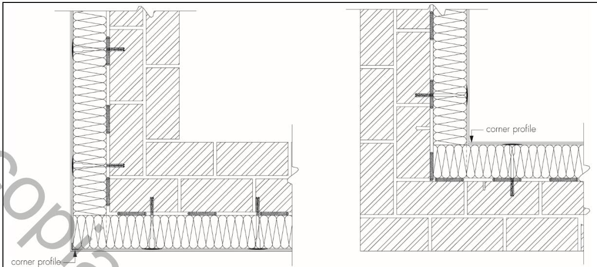
Figure 10 Corner details
