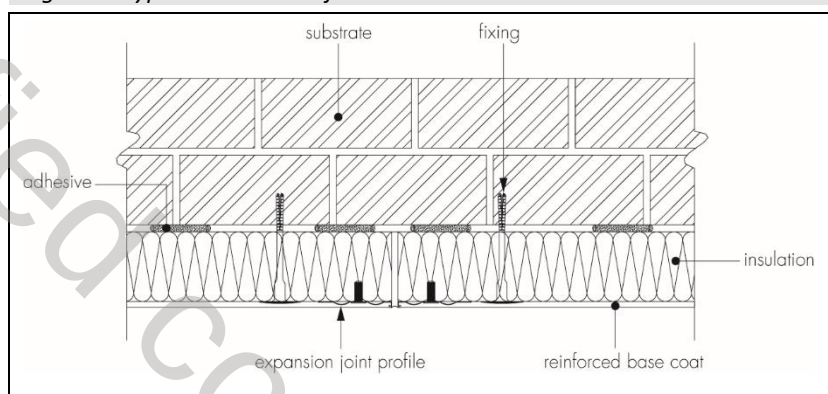
Figure 6 Typical movement joint
