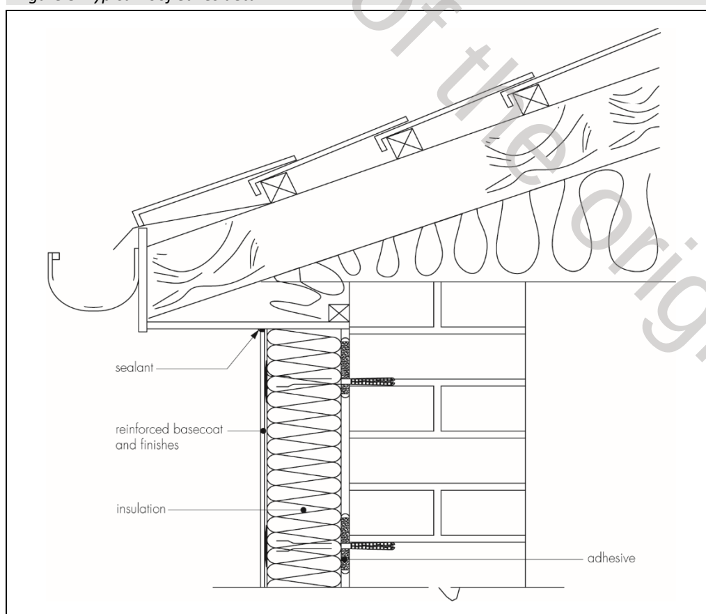
Figure 8 Typical roof eaves detail
