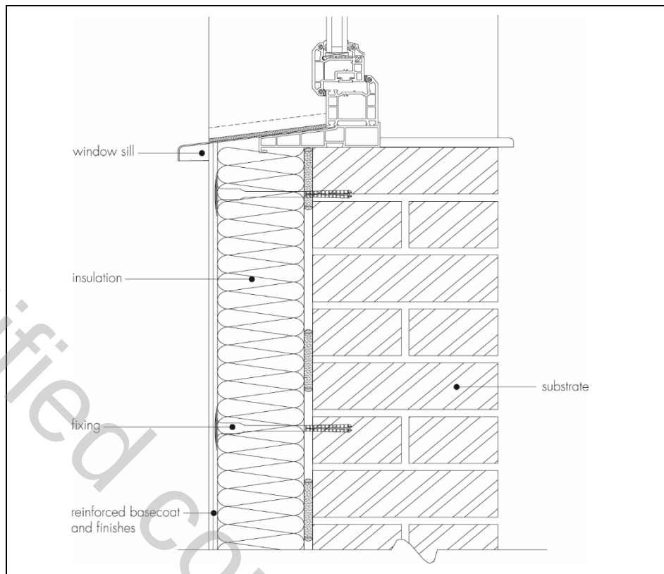
Figure 11 Window sill details
