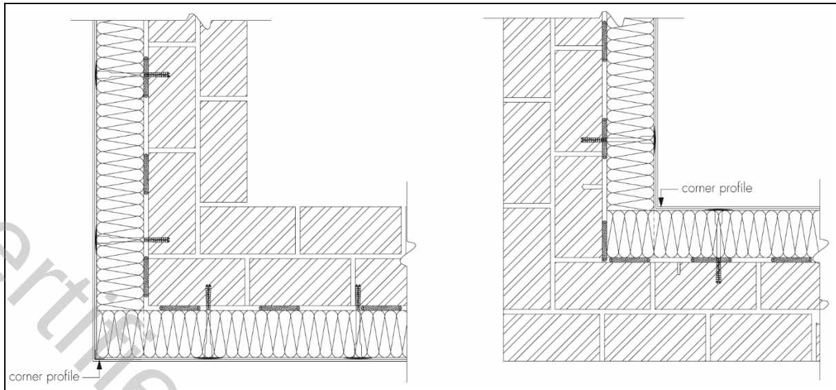
Figure 11 Corner details
