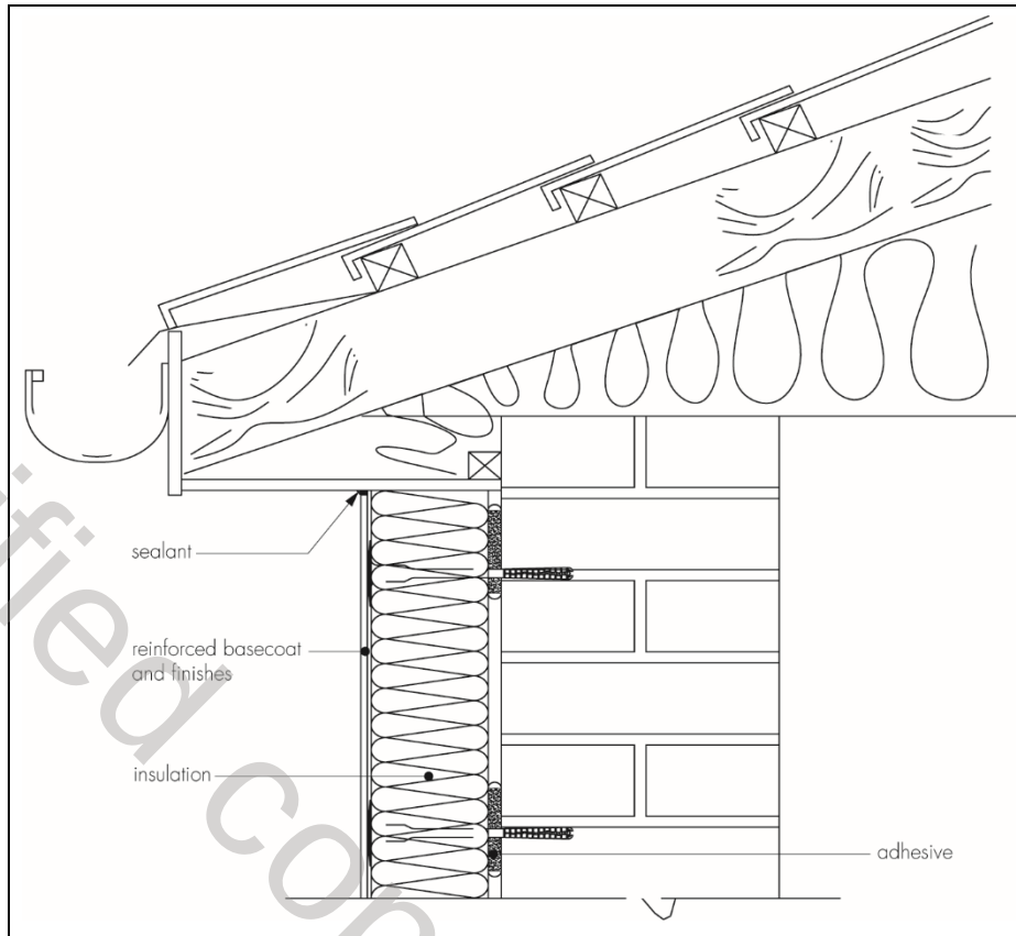
Figure 9 Typical roof eaves details
