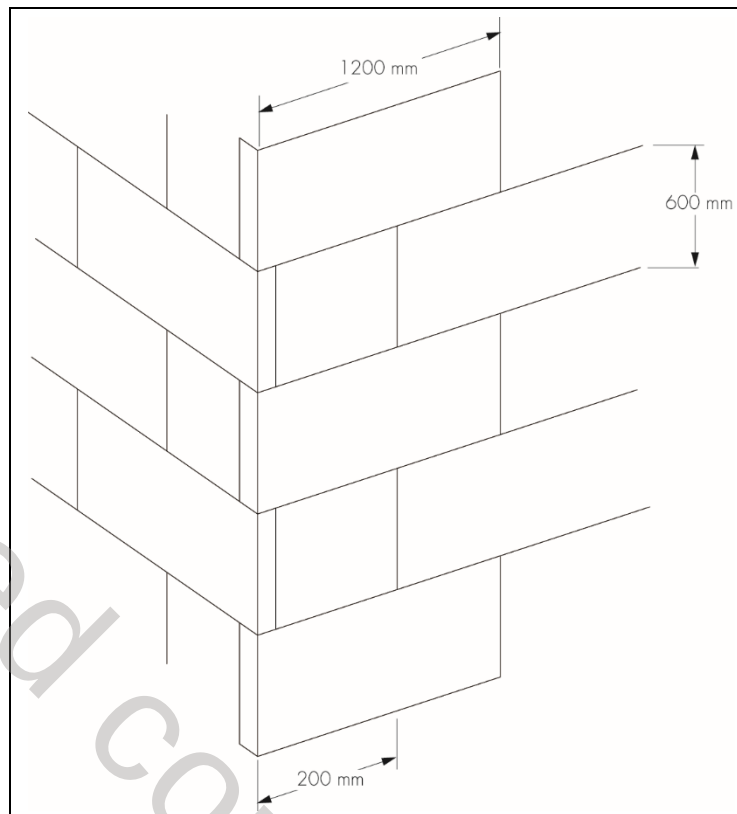
Figure 4 Typical arrangement of insulation boards
