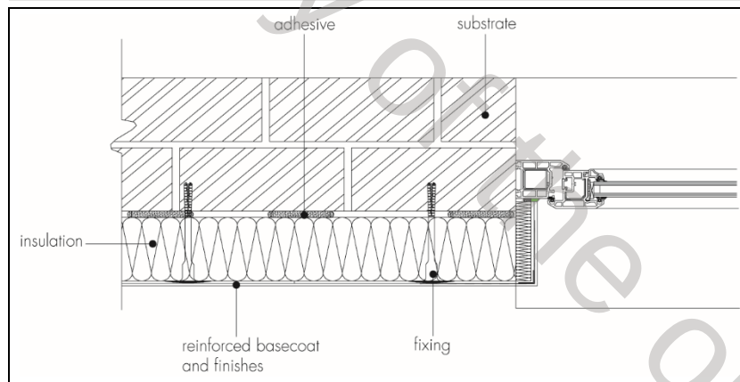
Figure 10 Window head details
