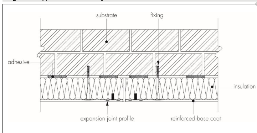
Figure 5 Typical movement joint
