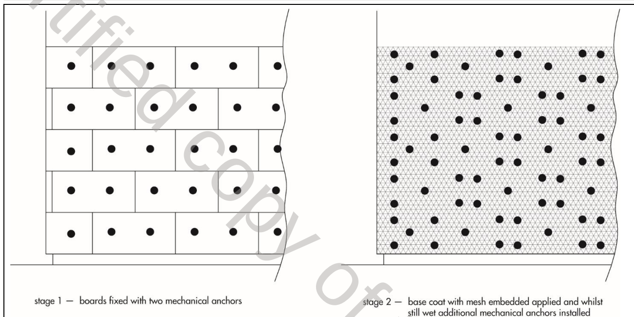
Figure 8 60-year durability fixings pattern
