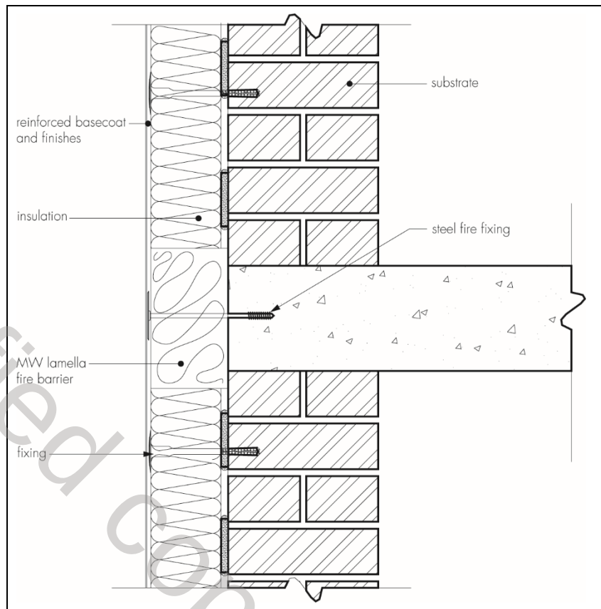
Figure 2 Fire barrier
