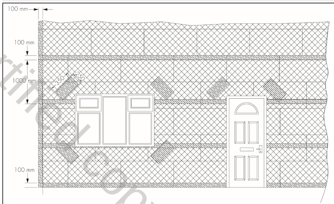
Figure 6 Reinforcement at openings
