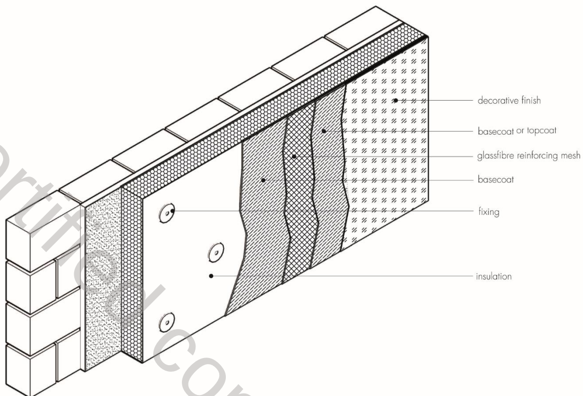
Figure 1 Termok8 Mechanically Fixed External Wall Insulation Render Systems – 60 Year
