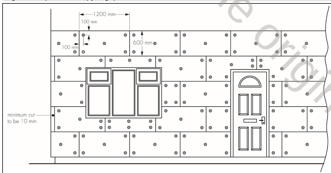
Figure 7 30-year durability fixings pattern
