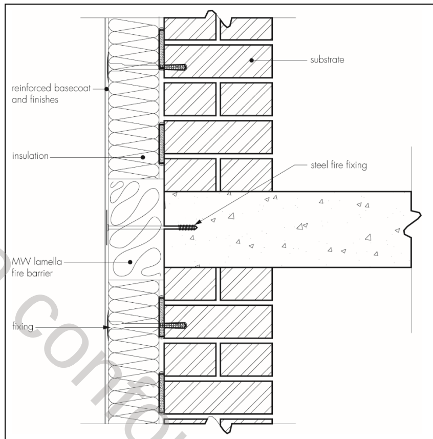
Figure 2 Fire barrier
