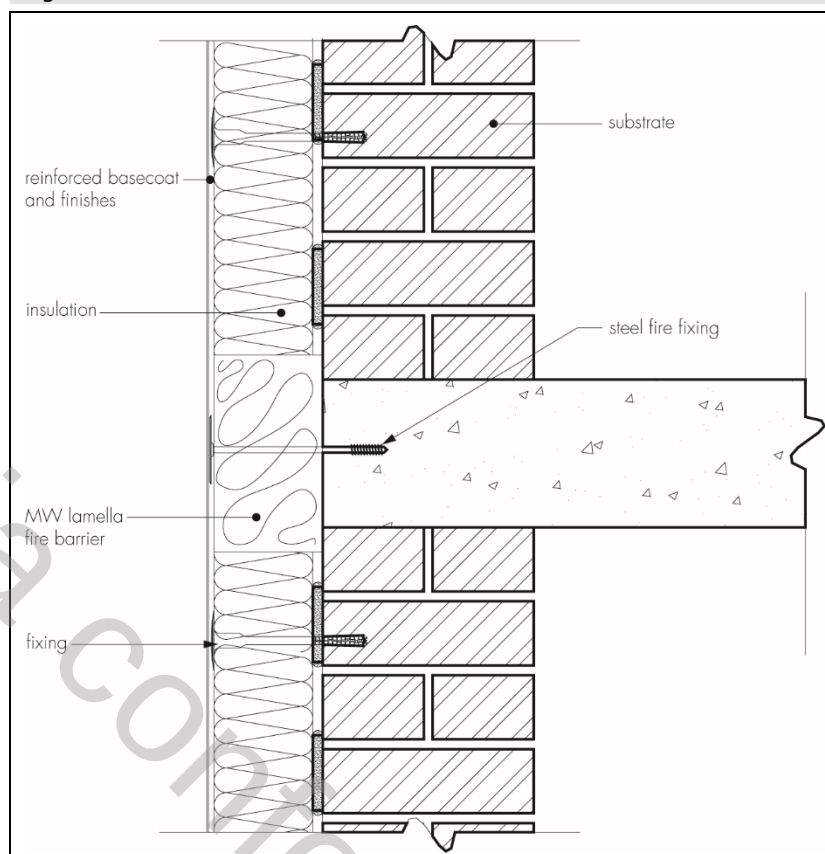
Figure 2 Fire barrier
