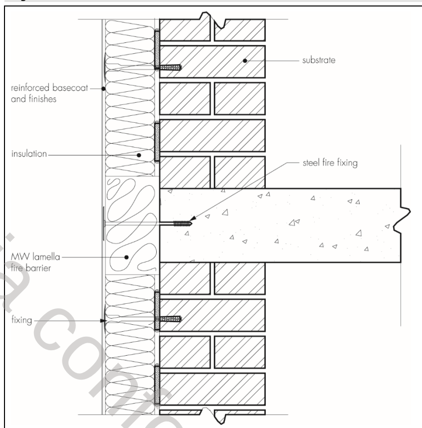
Figure 2 Fire barrier
